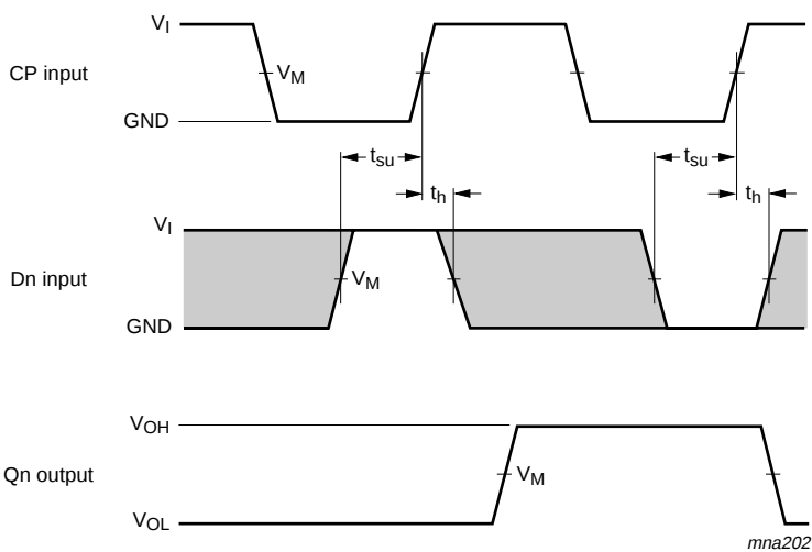
Measurement points are given in Table 8 . The shaded areas indicate when the input is permitted to change for predictable output performance. V_{OL} and V_{OH} are typical output voltage levels that occur with the output load.
